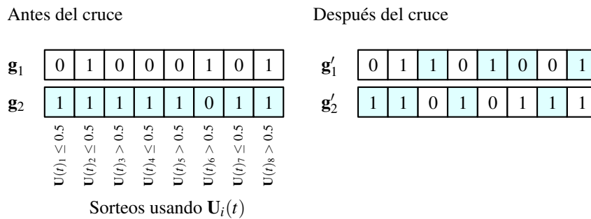
Figura 7.13: Crossover uniforme
